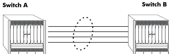
Static Aggregate Group 1 VLAN 8 with 802.1Q tagging has been configured to use this group.
