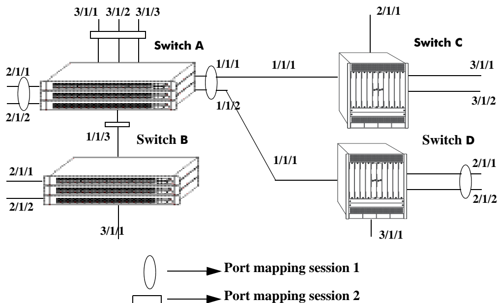
Example Port Mapping Topology
