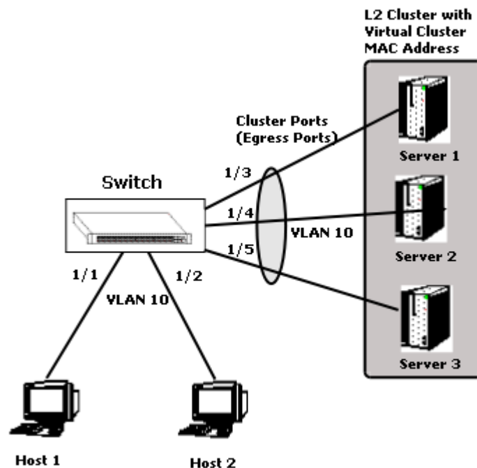
Switch connected to an L2 server cluster through 3 ports (1/1/3, 1/1/4, 1/1/5)
